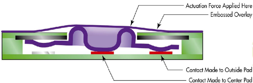
MagnaMouse™ (Cutaway View)
